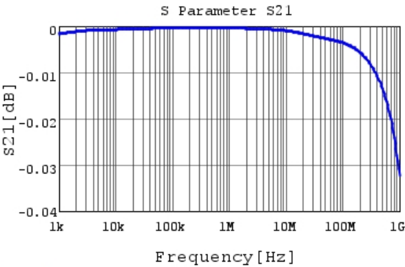
ECASD40E477M006KA0 S21 DCOV, 25degC
