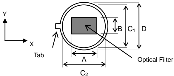
Fig.13 Top view
