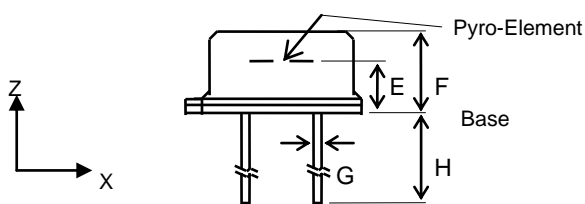
Fig.14 Side view
