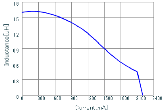
LQH3NPZ1R5MGR DC-Bias, 20
