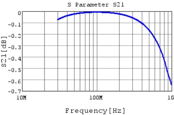
RHE5G1H391J0K1H03B S21 DCOV, 25degC
