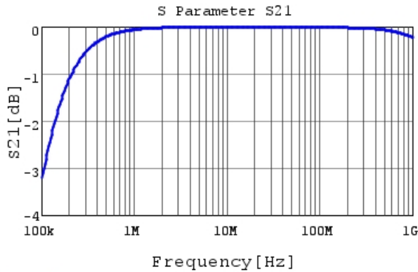
RHEL82A153K0DBH03A S21 DCOV, 25degC
