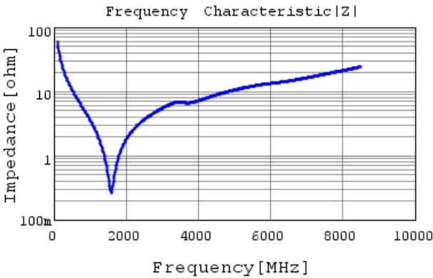
GCM1555C1H270JA16 |Z| DCOV,25degC
