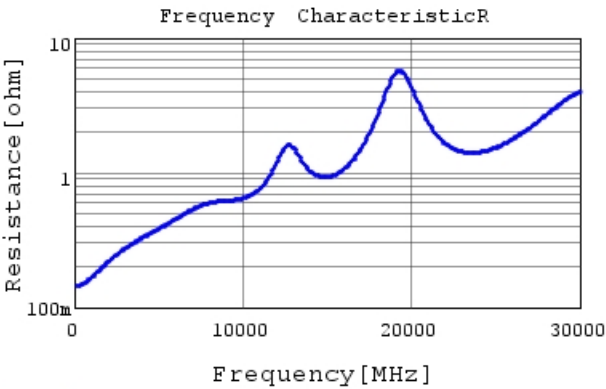
GRM0225C1H6R6CA03 R DCOV,25degC
