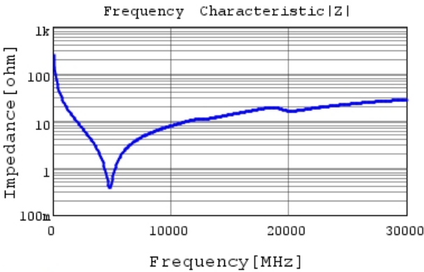
GRM0225C1H6R6CA03 |Z| DCOV,25degC
