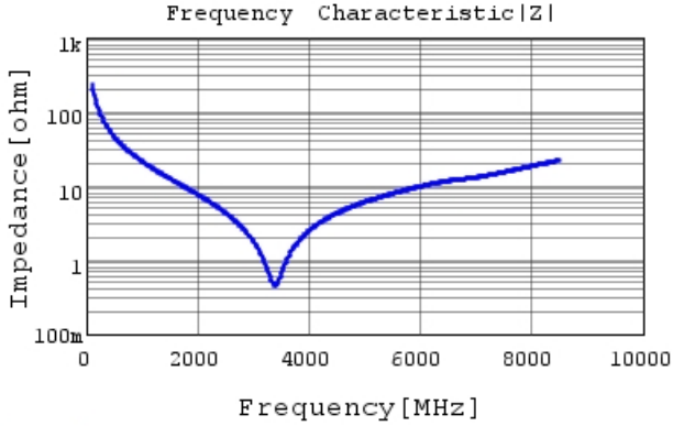
GRM1552C2A6R8DA01 |Z| DCOV, 20degC
