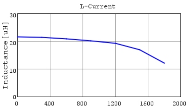
1253AY-220M L-Current 20degC
