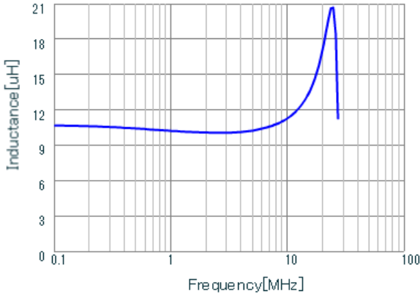
LQH3NPN100MGR L
