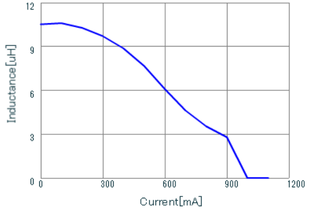
LQH3NPN100MGR DC-Bias, 20
