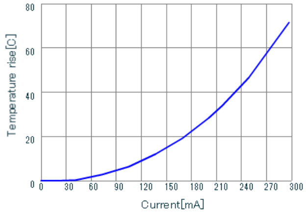
LQH3NPN181MGR DT_Current
