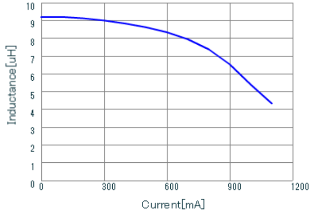
LQH44PZ100MGR DC-Bias, 20
