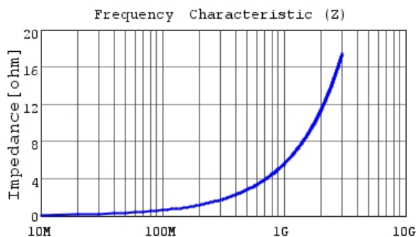
LQP03TG0N9C02 |Z|
