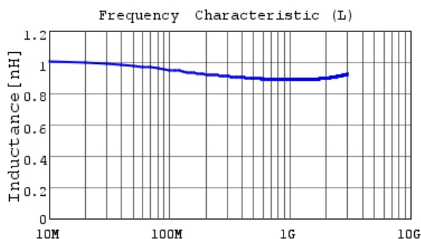
LQP03TG0N9C02 L
