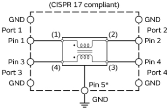
Equivalent Circuit
