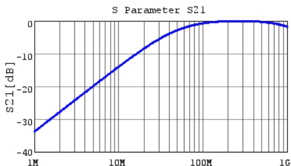
DE11XKX330JB4BC05F S21 DCOV, 20degC
