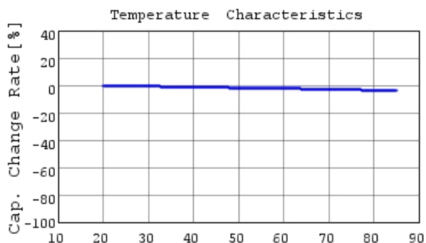
DE11XKX330JB4BC05F C-Temp. capchange, DCOV,
