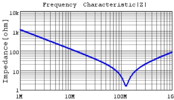
DE1B3RA151KJ4BQ01F |Z| DCOV, 20degC
