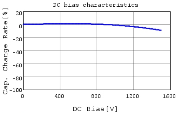
DE1B3RA151KJ4BQ01F C-DC bias capchange, 20.0
