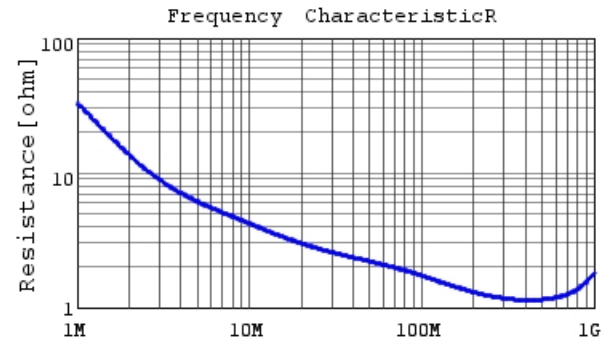
DE1B3RA151KJ4BQ01F R DCOV, 20degC
