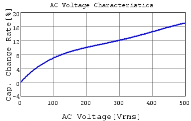
DE1B3RA151KJ4BQ01F C-AC Voltage capchange, 1
