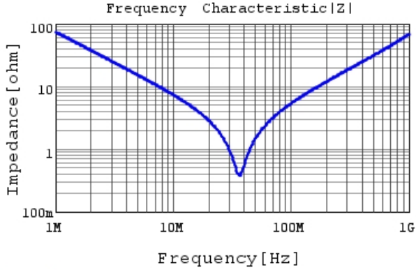
DE2E3SA222MN3AT02F |Z| DCOV, 20degC
