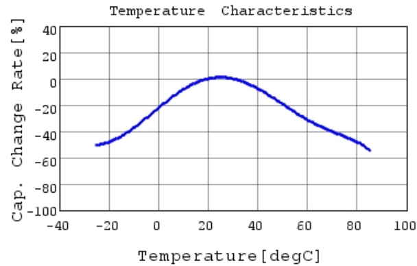
DE2E3SA222MN3AT02F C-Temp. capchange, DC0V,
