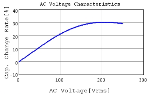
DE2E3SA222MN3AT02F C-AC Voltage capchange, I
