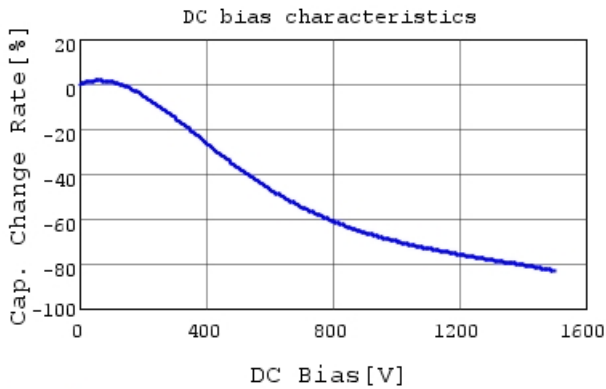
DE2E3SA222MN3AT02F C-DC bias capchange, 20.0
