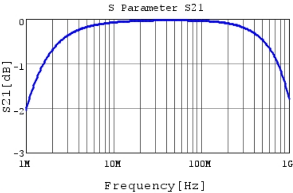
DE2E3SA222MN3AT02F S21 DC0V, 20degC
