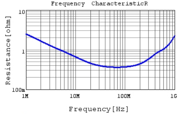
DE2E3SA222MN3AT02F R DCOV, 20degC
