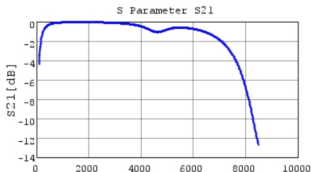
GRM1885C1H120JA01 S21 DCOV, 25degC
