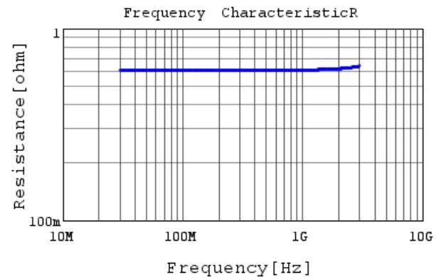
RCE5C1H1R0C0M1H03A R DCOV, 25degC
