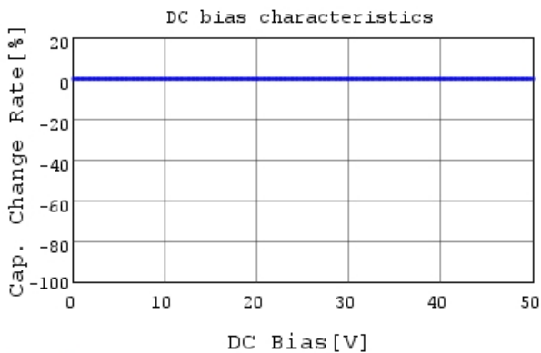
RCE5C1H1R0C0M1H03A C-DC bias capchange, 25.0
