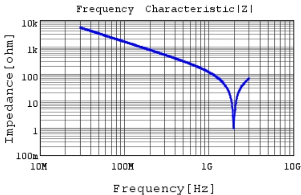
RCE5C1H1R0C0M1H03A |Z| DCOV, 25degC
