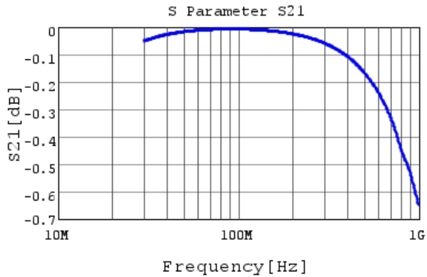
RHE5G1H471J0K1H03B S21 DCOV, 25degC
