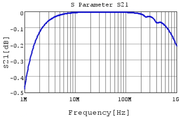
RHE5G1H472J1A2H03B S21 DCOV, 25degC
