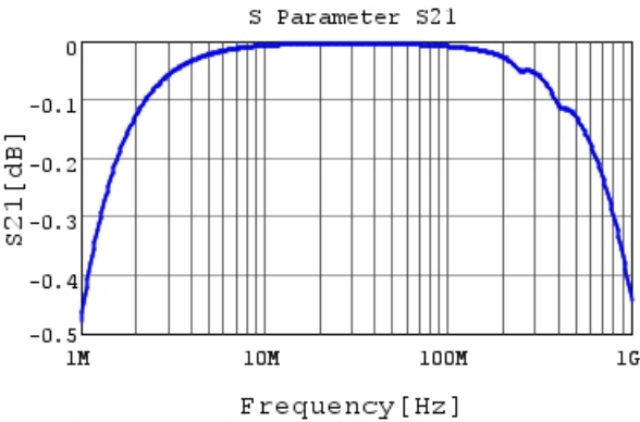
RHE5G1H472J1K1H03B S21 DCOV, 25degC
