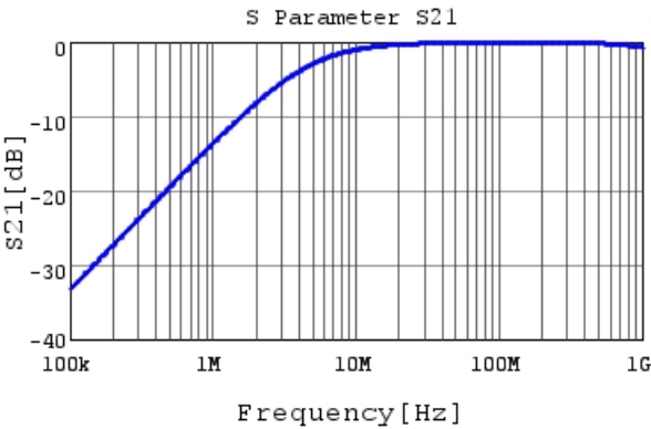
RHEL81H331K0M1H03A S21 DCOV, 25degC
