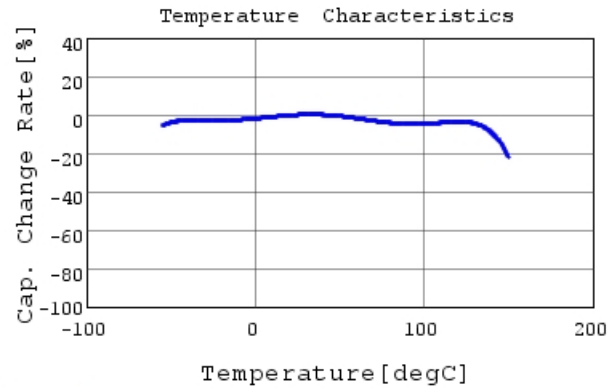
RHEL82A331K0M1H03A C-Temp. capchange, DCOV,
