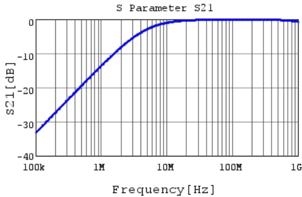
RHEL82A331K0M1H03A S21 DCOV, 25degC
