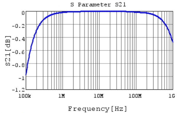
RHEL82A333K1M1H03A S21 DCOV, 25degC
