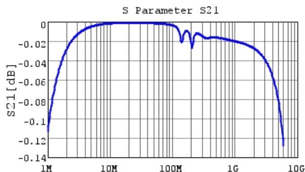
Frequency [Hz] GCM1885C1H103GA16 S21 DCOV, 25degC
