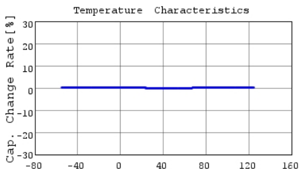
Temperature [degC] GCM1885C1H103GA16 C-Temp. capchange, DCOV, 1
