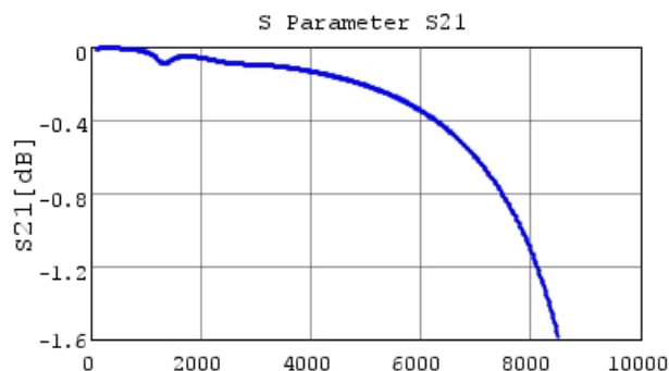
Frequency [MHz] GCM1885C2A331JA16 S21 DCOV, 25degC
