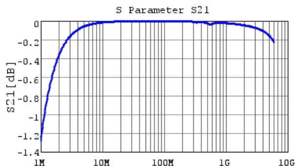
Frequency [Hz] ■ GCM1887U1H272JA16 S21 DCOV, 25degC
