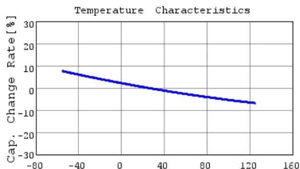
Temperature [degC] ■ GCM1887U1H272JA16 C-Temp. capchange, DCOV, 1
