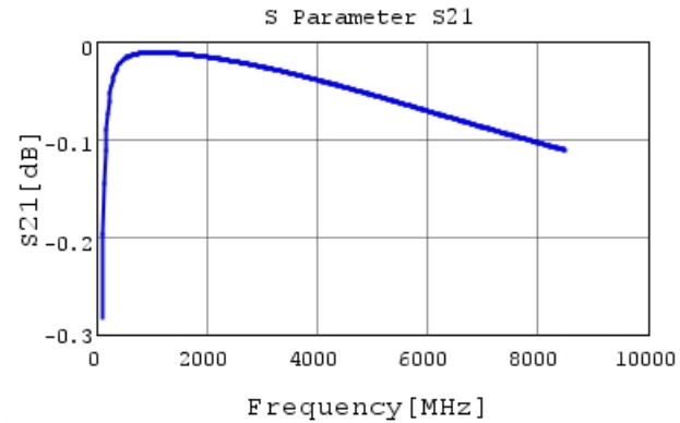
GRM0115C1C620JE01 S21 DCOV, 25degC
