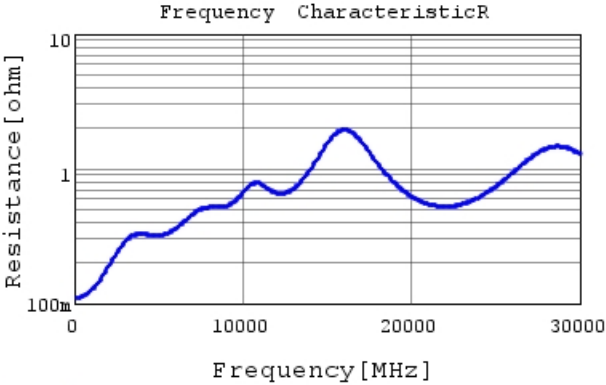
GRM0115C1E160GE01 R DCOV,25degC
