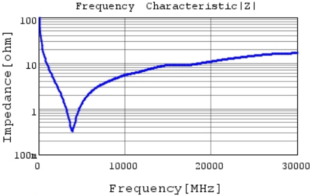
GRM0115C1E160GE01 |Z| DCOV,25degC
