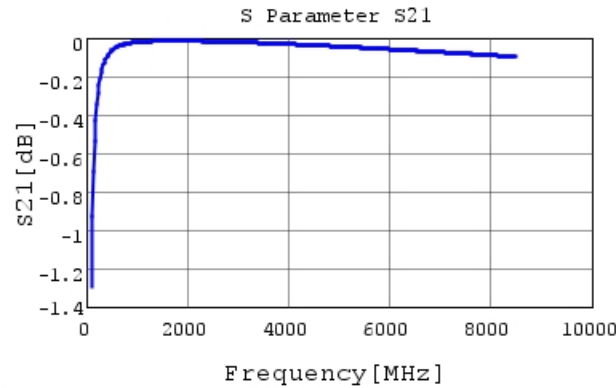
GRM0115C1E270GE01 S21 DCOV, 25degC
