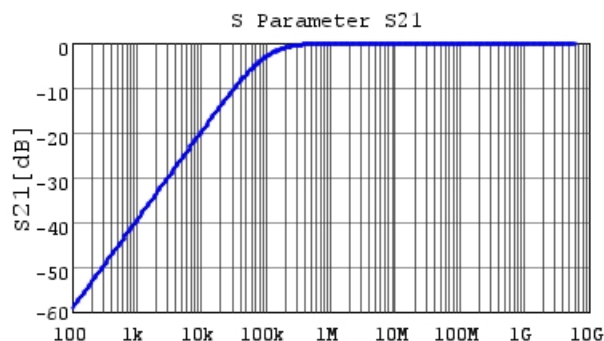
GRM011C80E223KE01 S21 DC0V,25degC
