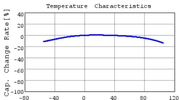
GRM011C80E223KE01 C-Temp. capchange, DC0.0V,
