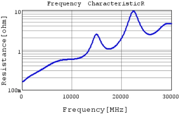
GRM0225C1H4R5WA03 R DCOV, 25degC
