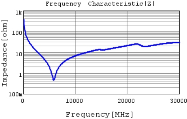
GRM0225C1H4R5WA03 |Z| DCOV, 25degC
