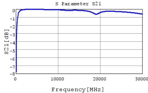
GRM0225C1H7R1DA03 S21 DCOV, 25degC
