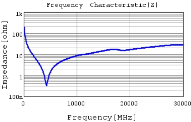
GRM0225C1H8R4WA03 |Z| DCOV,25degC
