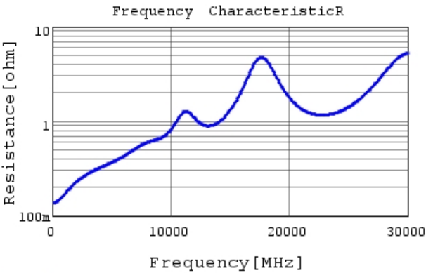
GRM0225C1H8R4WA03 R DCOV,25degC
