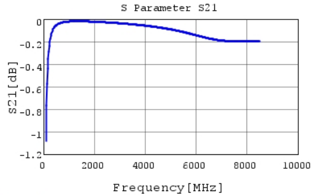
GRM0332C2A300JA01 S21 DCOV, 20degC
