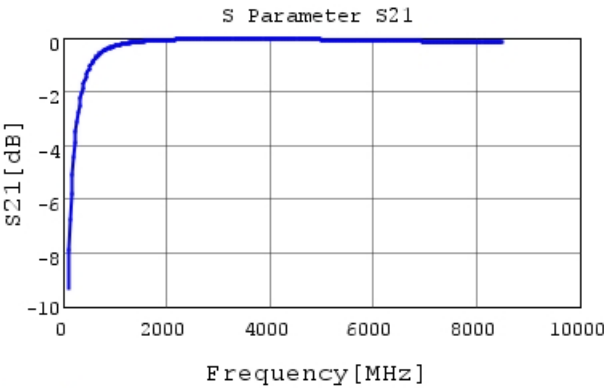
GRM0335C1H5R8WA01 S21 DCOV, 25degC
