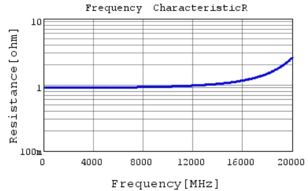
GRM1554C2AR30WA01 R DCOV, 20degC
