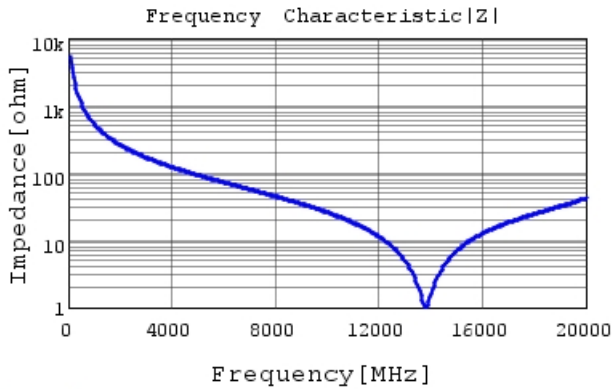
GRM1554C2AR30WA01 |Z| DCOV, 20degC
