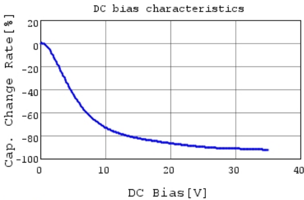
GRM188R6YA475ME15 C-DC bias capchange, 25.0C
