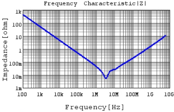
GRM188R6YA475ME15 |Z| DCOV,25degC
