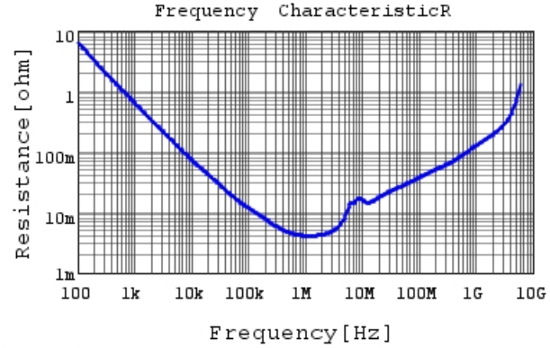
GRM188R6YA475ME15 R DCOV,25degC
