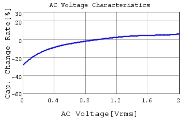
GRM188R6YA475ME15 C-AC Voltage capchange, D
