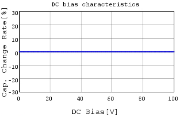
GRT1885C2A120JA02 C-DC bias capchange, 25.0C
