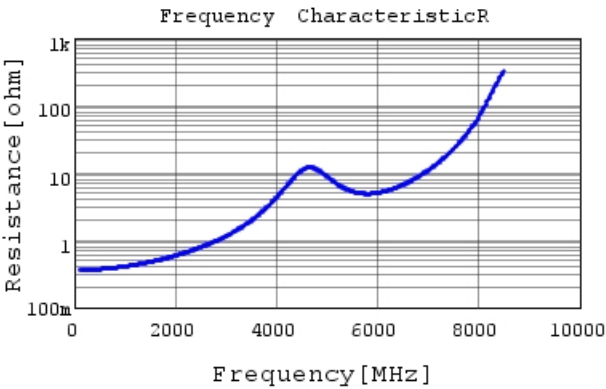
GRT1885C2A120JA02 R DCOV, 25degC
