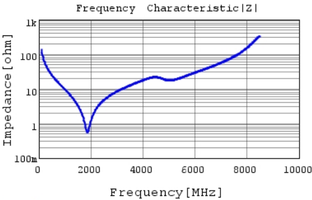
GRT1885C2A120JA02 |Z| DCOV, 25degC
