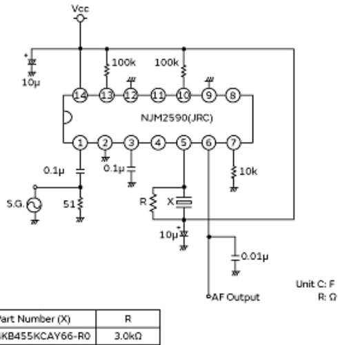
Measurement Circuit
