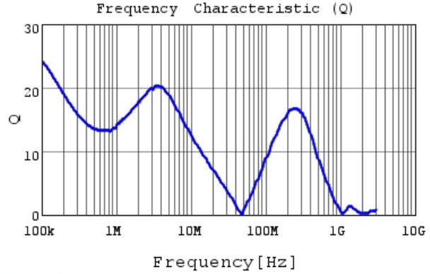
1253AY-6R8M Q
