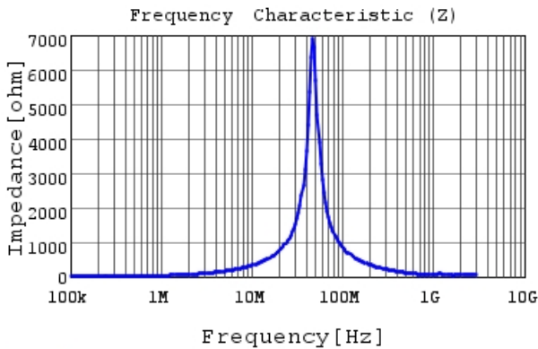
1253AY-6R8M |Z|
