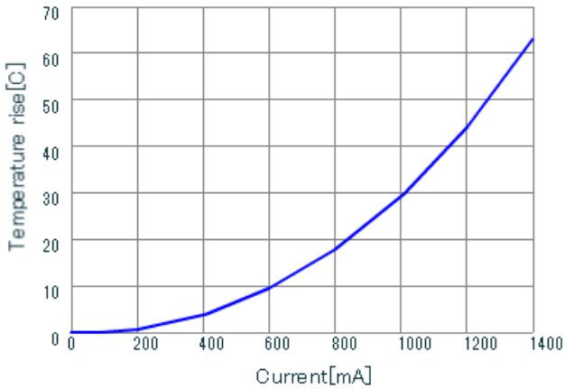
LQH2HPN6R8MJR DT_Current
