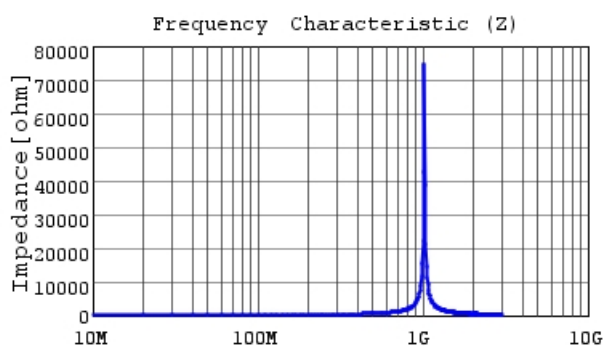
LQW2UASR15G00 |Z|
