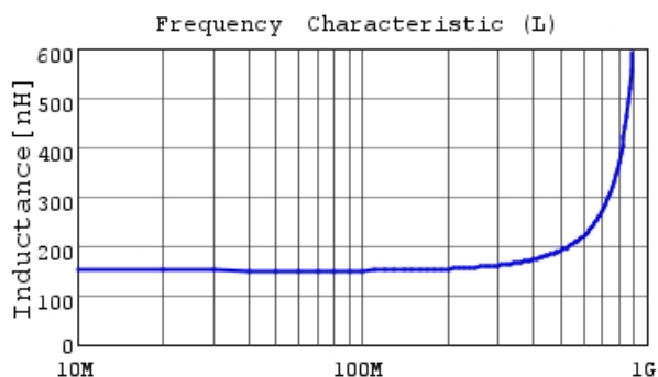
LQW2UASR15G00 L
