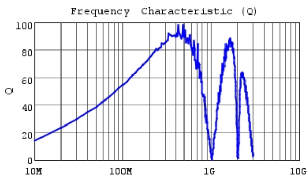
LQW2UASR15G00 Q
