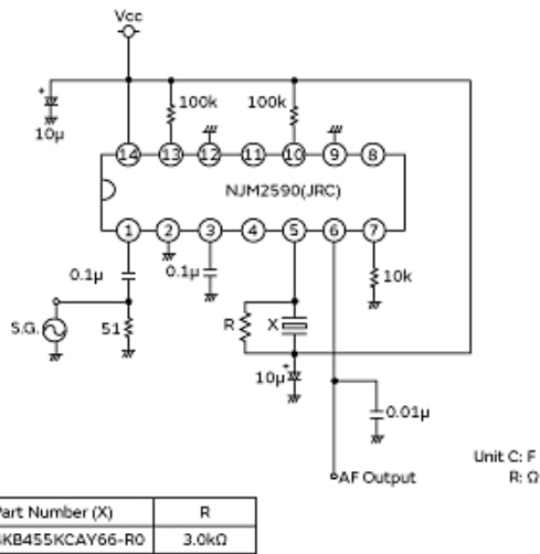
Measurement Circuit
