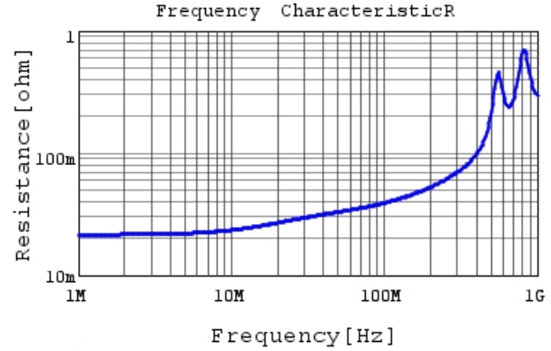
RHE5G1H102J0A2H03B R DCOV, 25degC
