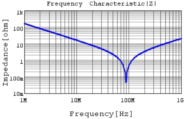
RHE5G1H102J0A2H03B |Z| DCOV, 25degC
