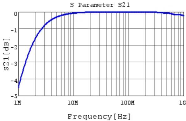
RHE5G1H122J0A2H03B S21 DCOV, 25degC
