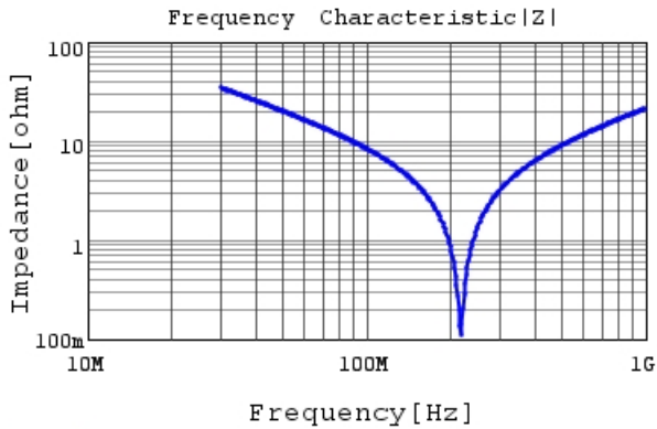
RHE5G2A151J0A2H03B |Z| DCOV, 25degC
