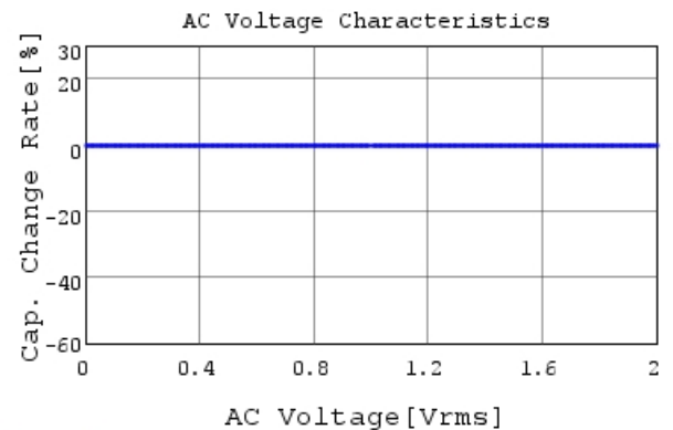
RHE5G2A151J0A2H03B C-AC Voltage capchange, I
