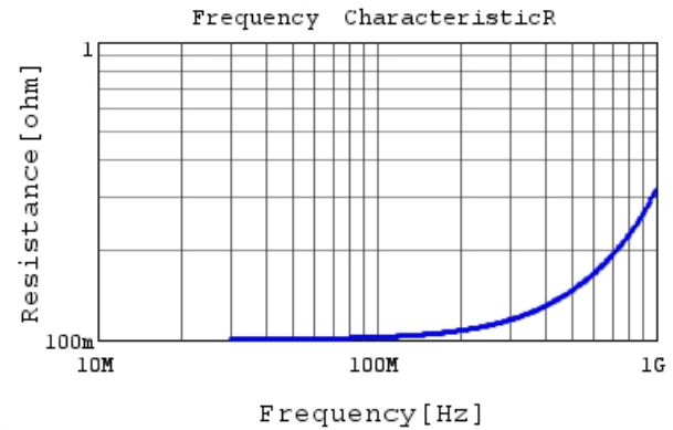
RHE5G2A151J0A2H03B R DCOV, 25degC
