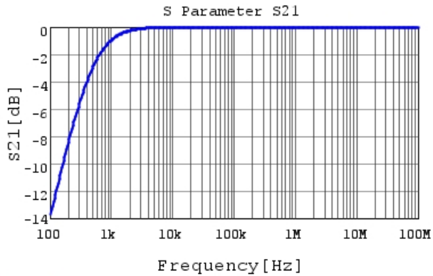
RHEL81H335K3DBH03A S21 DCOV, 25degC
