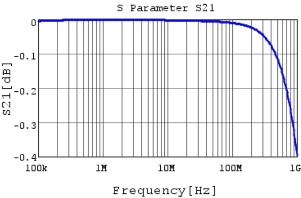
RHEL81H684K2DBH03A S21 DCOV, 25degC
